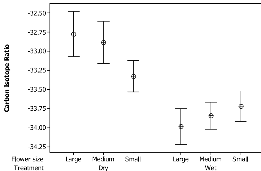
Fig. 1. The mean carbon isotope ratio ( \delta^{13}\text{C} value) is given for each flower size category in each experimental treatment. The bands define a 95% confidence interval on each mean.
