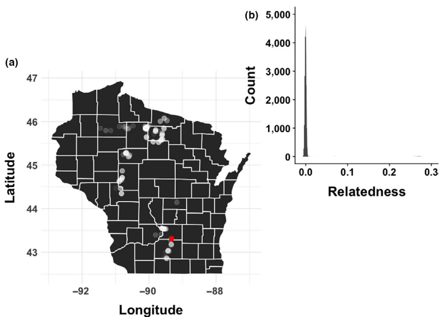
FIGURE 1 (a) Map of Wisconsin that displays the origin of the WisAsp aspen genets (white points, shown with 30% transparency) and the WisAsp common garden (red point). (b) Histogram of relatedness values (calculated using GEMMA, derived from a kinship matrix) for all pairwise comparisons of the 445 genets. Low values (0) indicate that the pair of genets is completely unrelated, whereas higher values (0.25) indicate that the pair of genets is more related and have a potential sibling relationship
