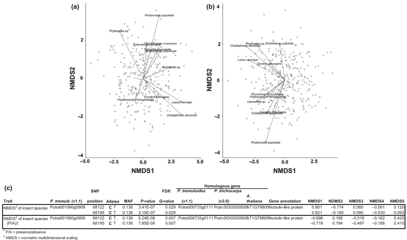
FIGURE 2 Nonmetric multidimensional scaling (NMDS) ordination for both the (a) abundance and (b) incidence of common insect species surveyed on aspen in the WisAsp common garden (2014–5). Each point represents an insect community on an aspen genet. Each vector shows the insect species-level changes in the community (i.e. along a given vector, the particular insect species is either more [a] abundant or more [b] present within the insect community). (c) Summary of significant single nucleotide polymorphism (SNP) associations (false discovery rate [FDR] q -value < 0.10) for multivariate insect phenotypes for the WisAsp Populus tremuloides genetic mapping population ( N = 328 genets). Genome-wide association models were analysed in PLINK without a kinship matrix. Bolded alleles are the minor allele
